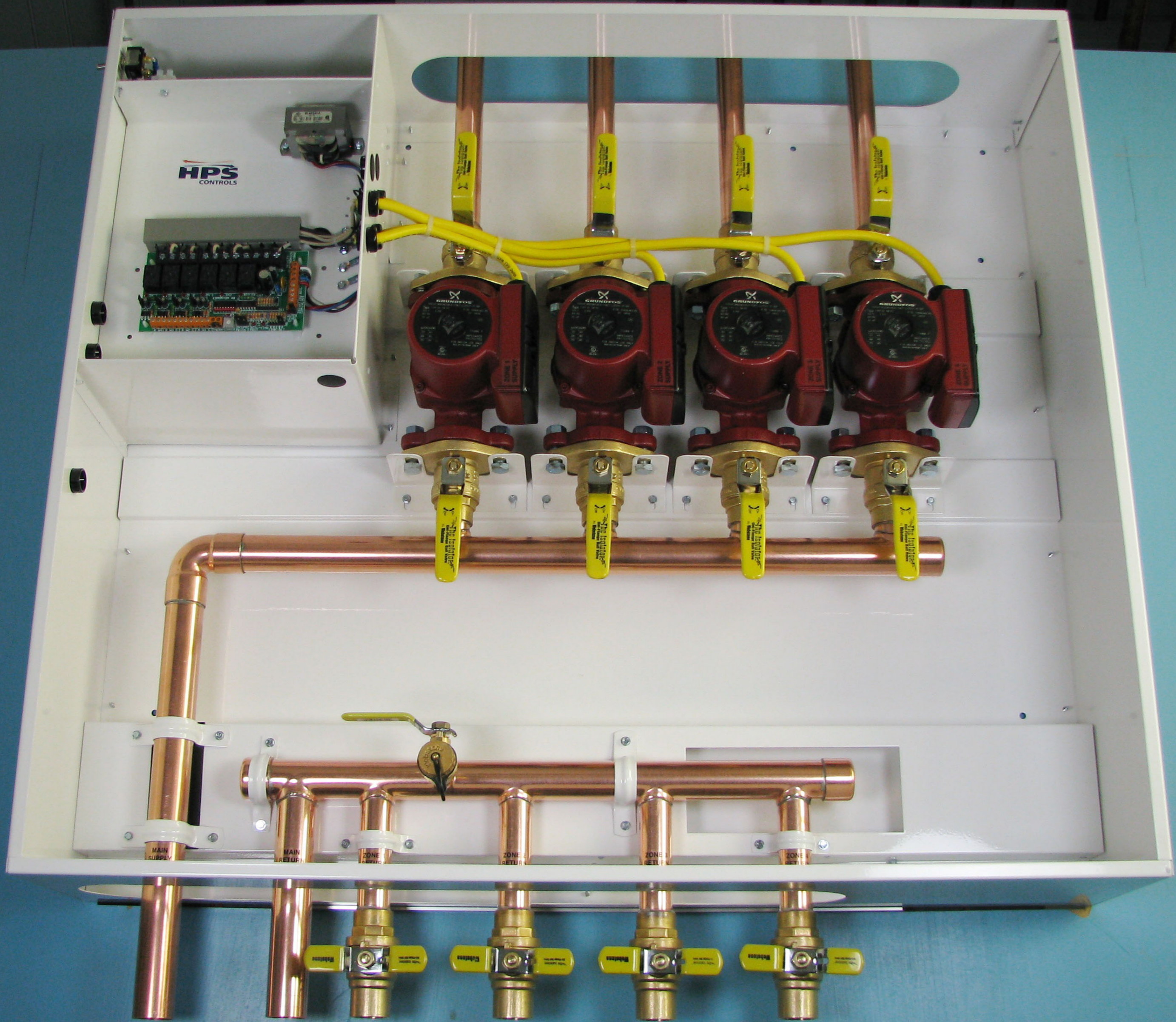
HFS-4 [High Temp 4 Zone Flange Pump Zone Control Station]
